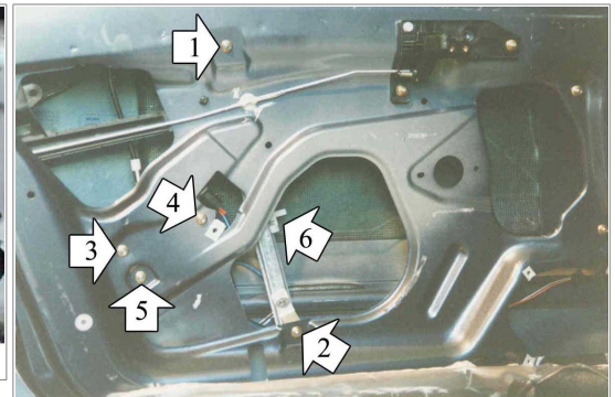
FIAT BRAVA 4 Doors - Front Doors
