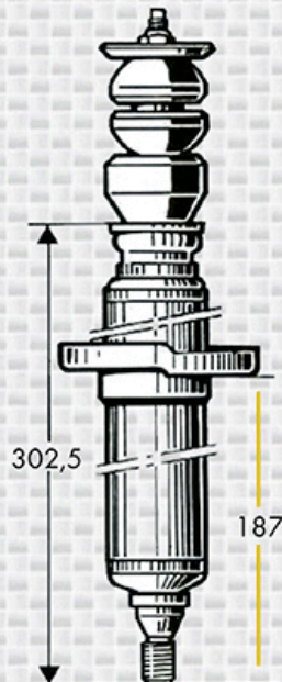
ORIGINAL R 6521 hydraulic shock absorber
