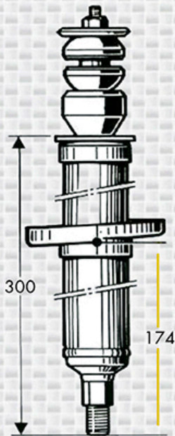
REFLEX E 5604 gas shock absorber
