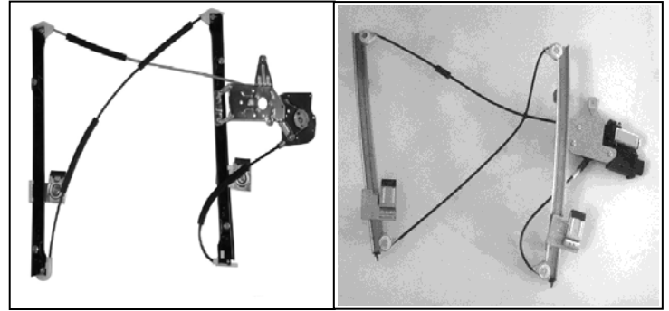
Elevavinas original Oem window regulator
