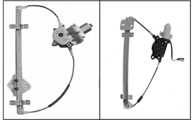
elevavinas original – oem window regulator
