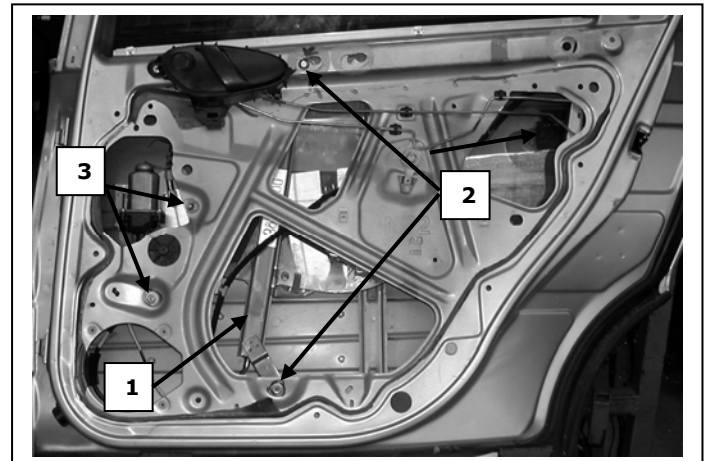
Porta lato destro, Portière arrière droite, Right rear door, Puerta lado derecho, Hinten rechte Tür, Porta traseira direita, Sag arka kapı, πόρτα οπίσθια δεξιά
