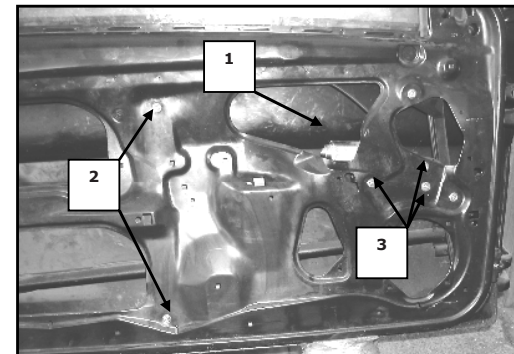
Porta lato destro, Portière avant droite, Right front door, Puerta lado derecho, Vorne rechte Tür, Porta frente direita, Sag on kapi, νόρτα εμπρόσθια δεξιά
