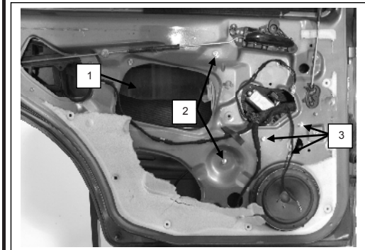
Porta lato destro, Portière arrière droite, Right rear door, Puerta lado derecho, Hinten rechte Tür, Porta traseira direita, Sag arka kapi, νότρο οπίσθιο δεξιά
